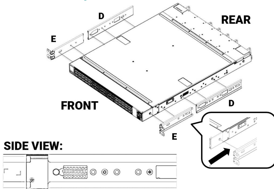
圖四：Server Rail Kit Design
